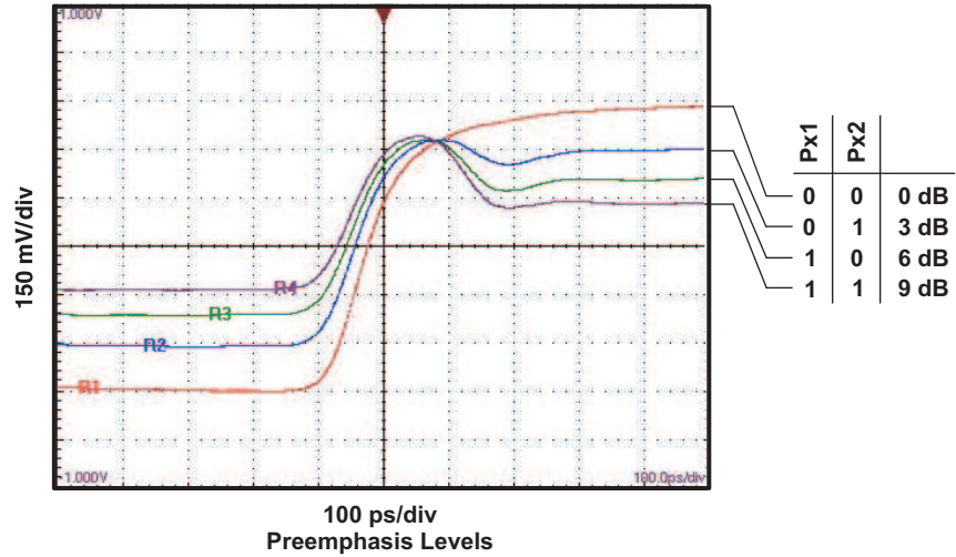
Figure 10. Preemphasis Signal Shape
