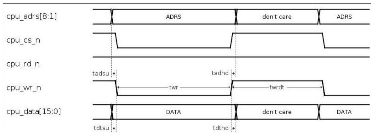
Figure 11 Host Interface, WRITE Timing
