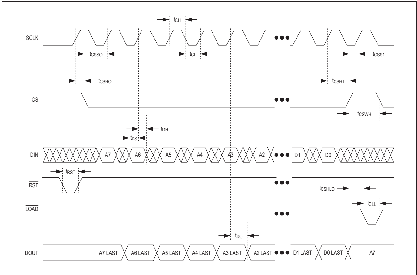
Figure 9. Serial-Interface Timing
