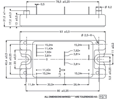
SP6–Four Outputs, Version 1
