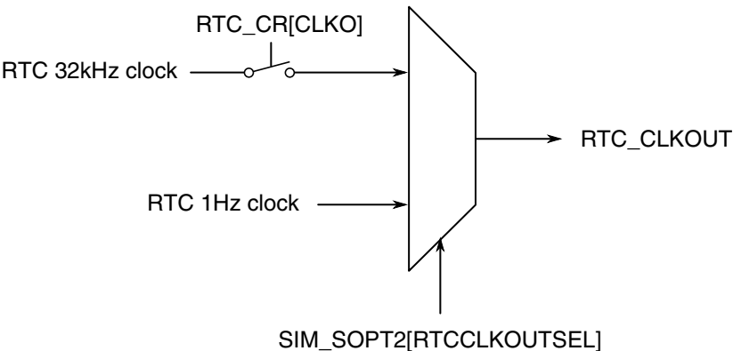
Figure 3-44. RTC_CLKOUT generation
