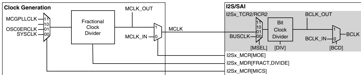
Figure 5-7. I²S/SAI clock generation
