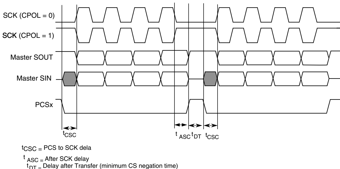
Figure 42-73. Example of non-continuous format (CPHA=1, CONT=0)
