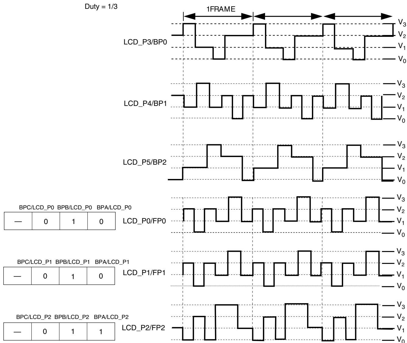
Figure 48-40. LCD waveforms
