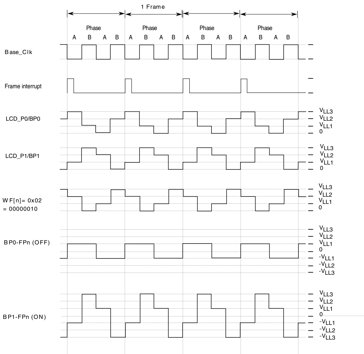
Figure 48-29. 1/2 duty and 1/3 bias (low-power waveform)
