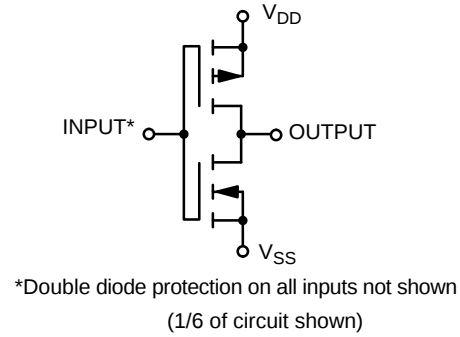
Figure 2. Circuit Schematic
