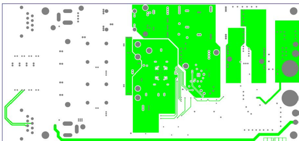
Figure 34. STEVAL-POE005V1 reference design PCB layer 3
