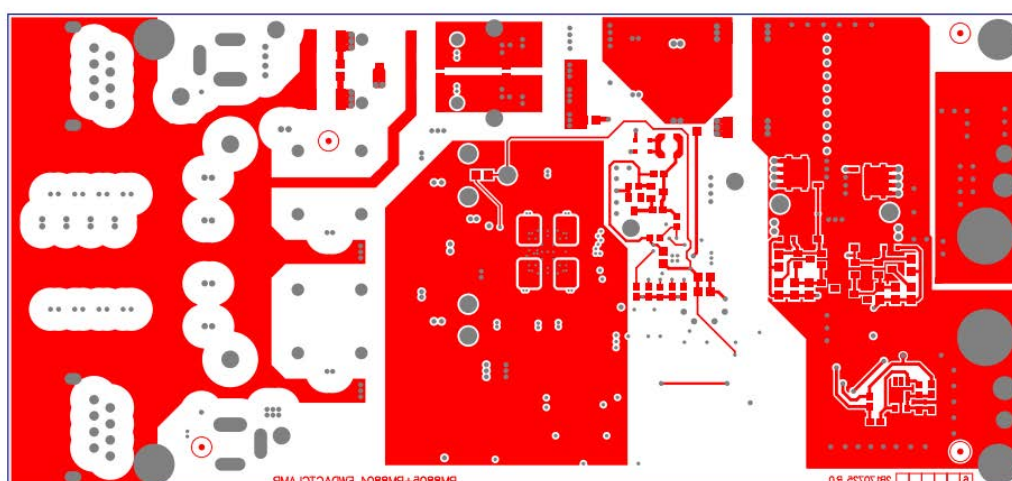
Figure 37. STEVAL-POE005V1 reference design PCB layer 6
