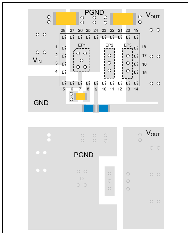
Figure 2. Layout Recommendation
