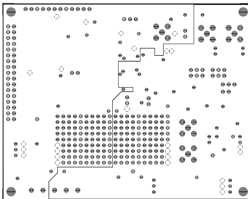
Figure 2-4. Board Layout, Layer 3
