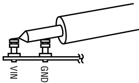
Figure 6. Measuring Input or Output Ripple
