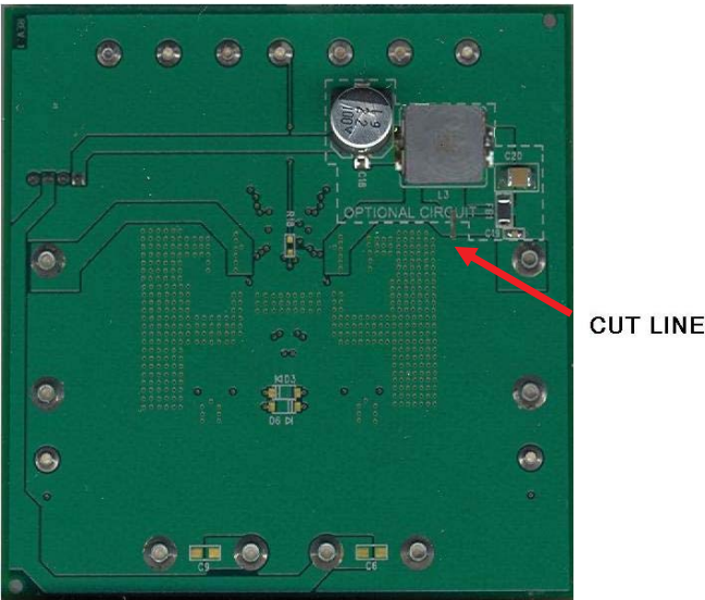
Figure 7. Cut Line for the EMI Filter Installation
