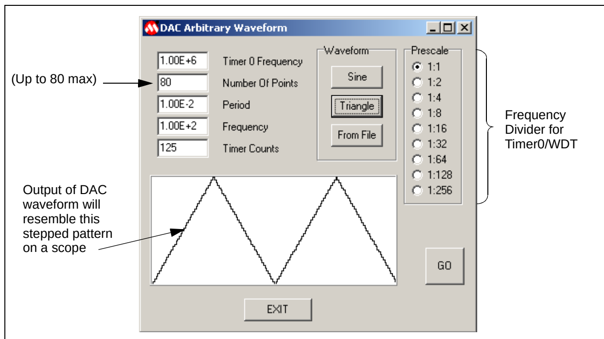
Figure 2.11: Triangle Waveform Example
