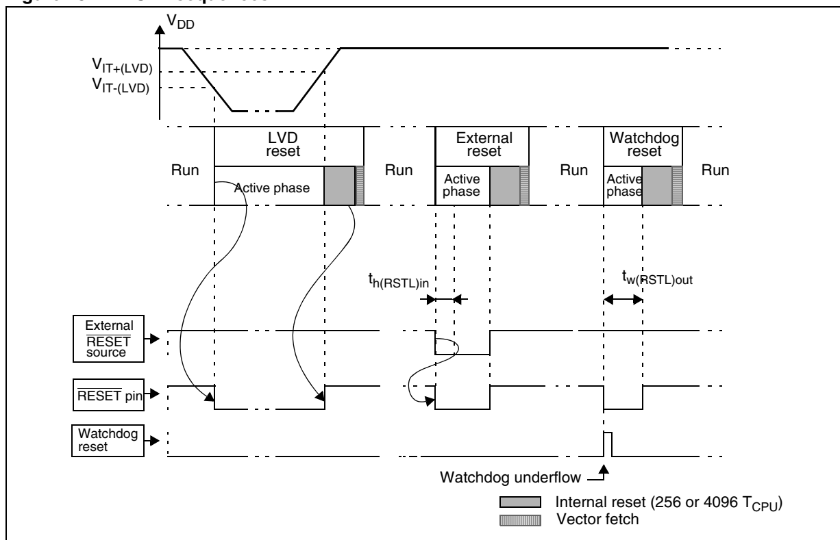
Figure 15. RESET sequences
