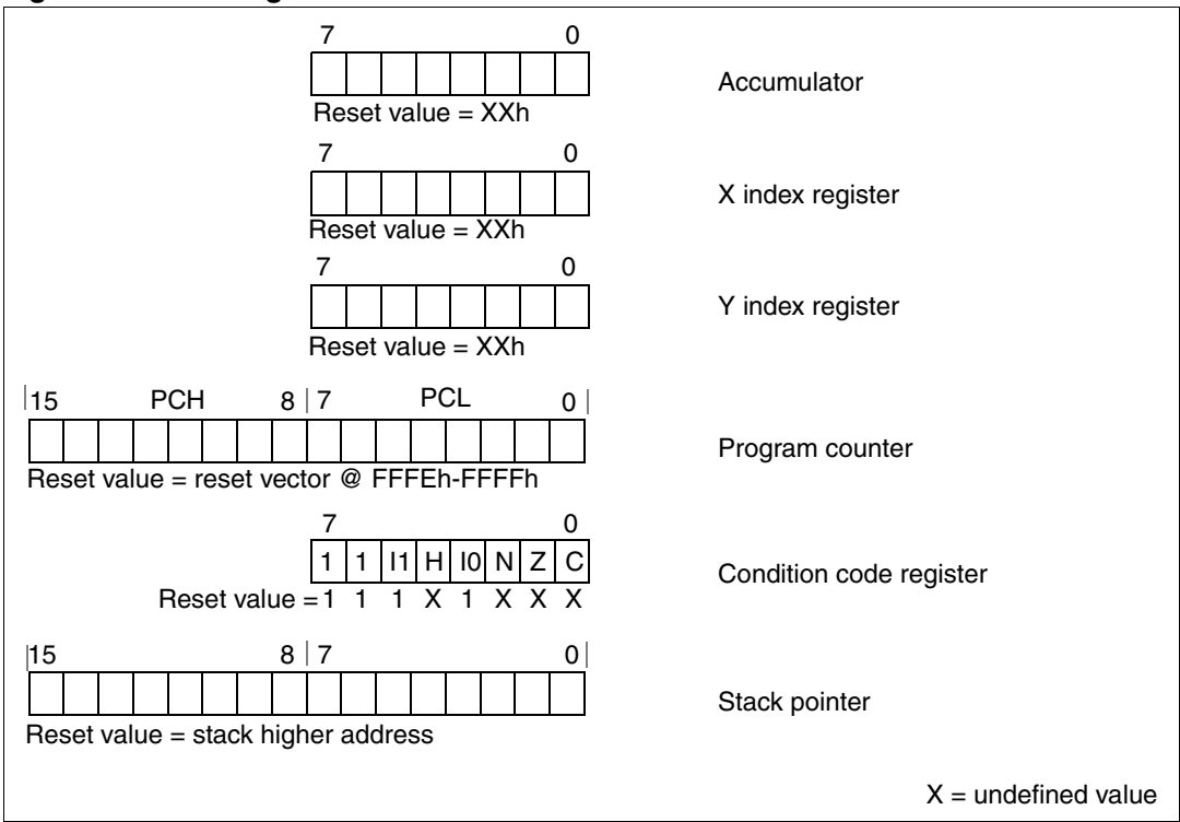
Figure 9. CPU registers
