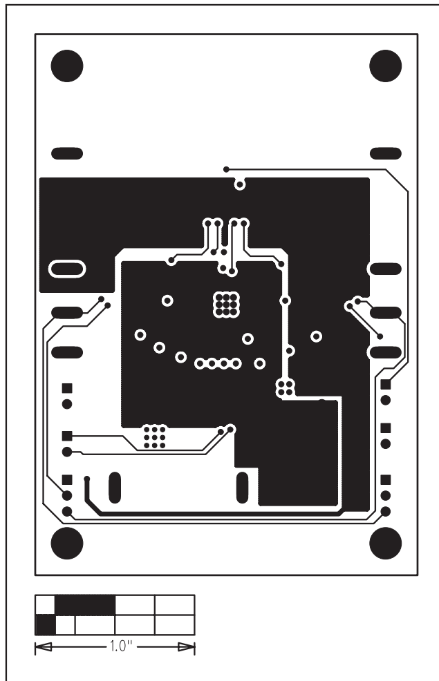
Figure 5. MAX5099 EV Kit PCB Layout—Layer 3 (Signal)
