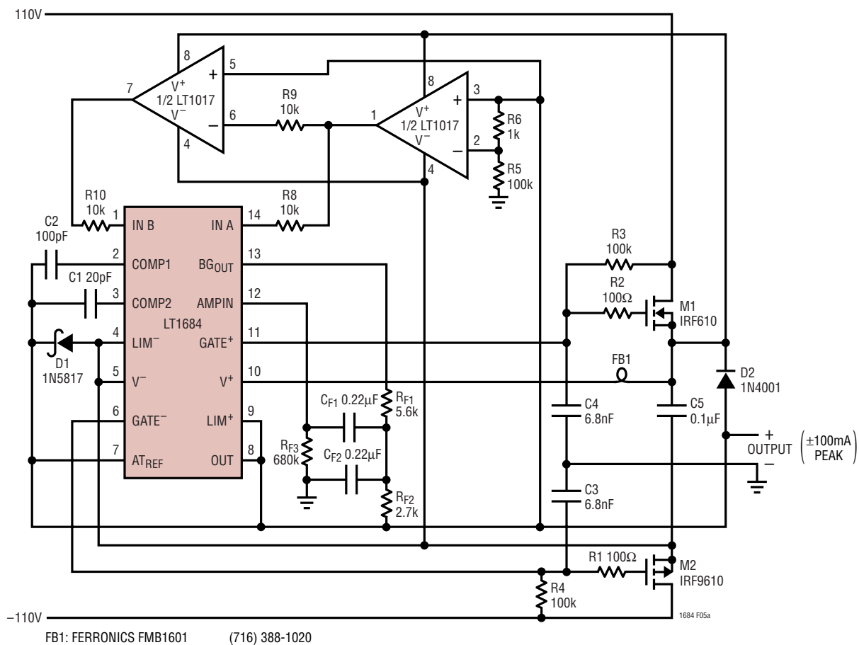
Active Filter Tuned Oscillator Ring Tone Generator
