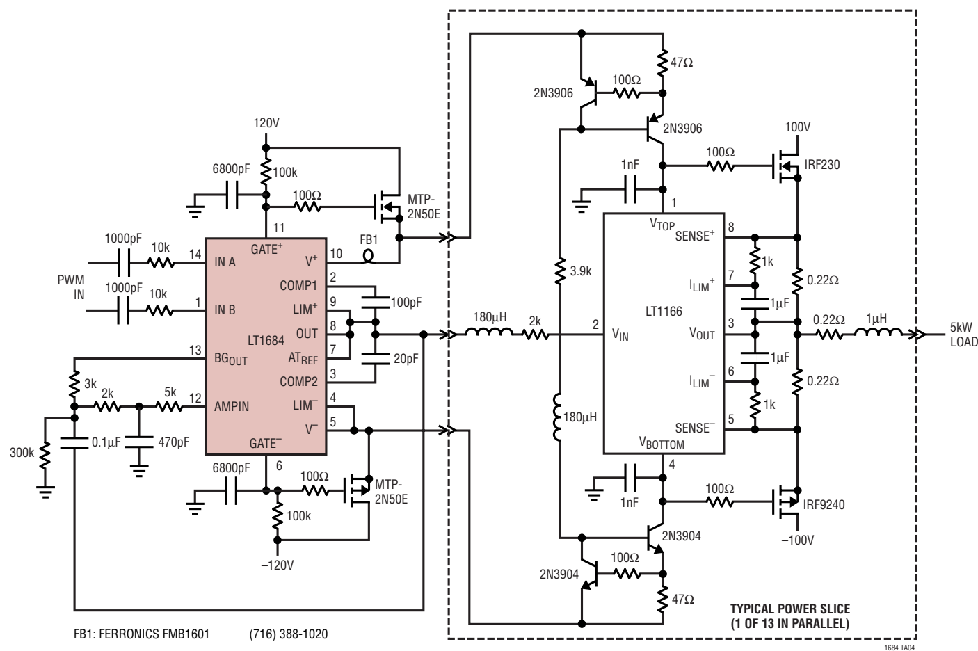
5kW PWM-to-Analog Converter
