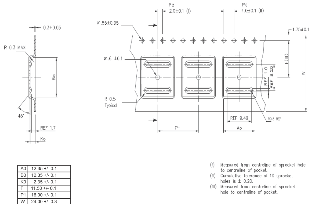
Figure 24. TQFP-64 power lead-less tape and reel shipment (suffix "TR") (part 1)
