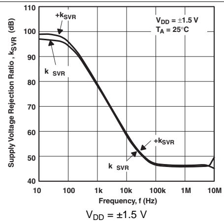
Figure 18. Supply-Voltage Rejection Ratio vs Frequency
