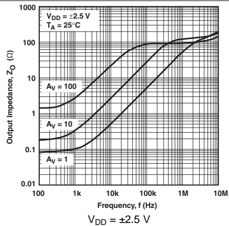
Figure 16. Output Impedance vs Frequency
