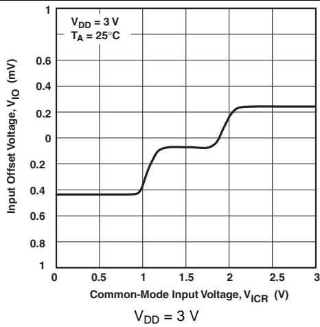
Figure 1. Input Offset Voltage vs Common-Mode Input Voltage
