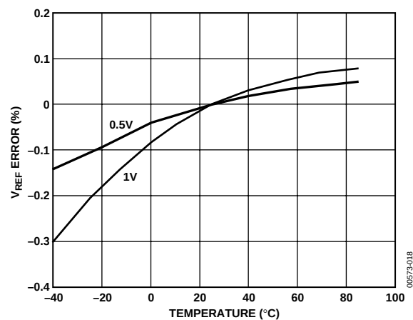
Figure 18. Reference Voltage vs. Temperature
