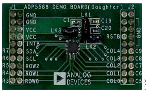
Figure 2. Daughterboard
