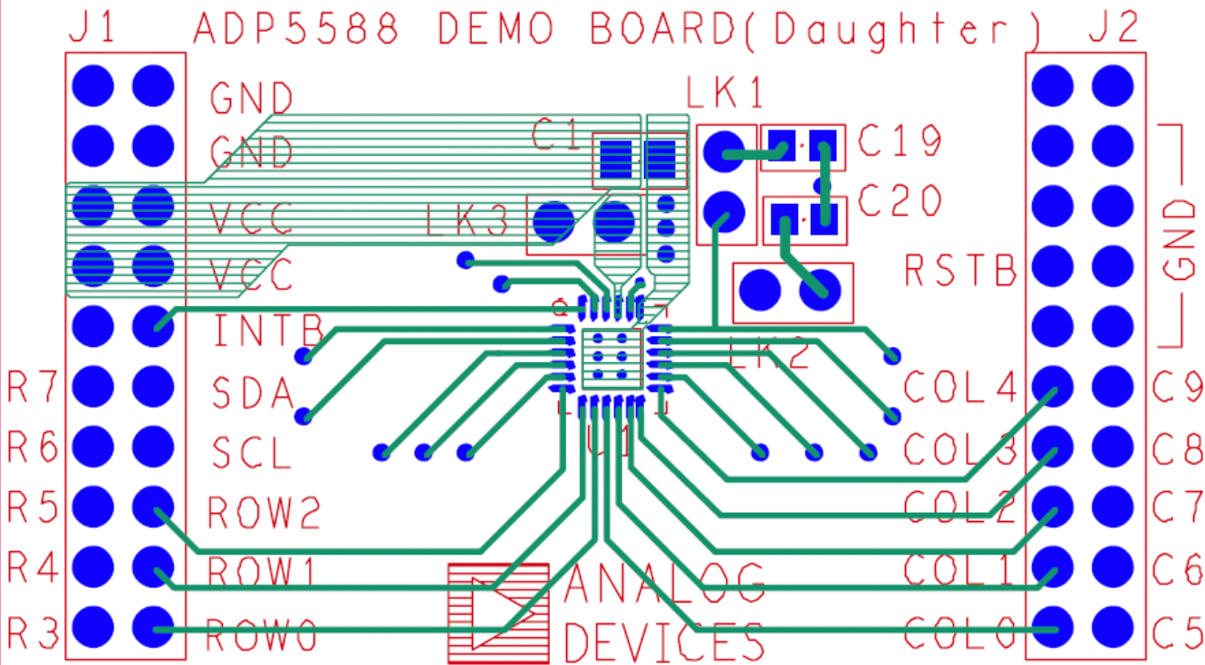
Figure 28. Daughterboard Layout (Top Layer)
