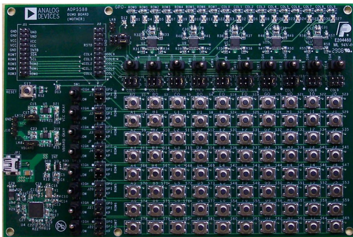
Figure 3. Motherboard
