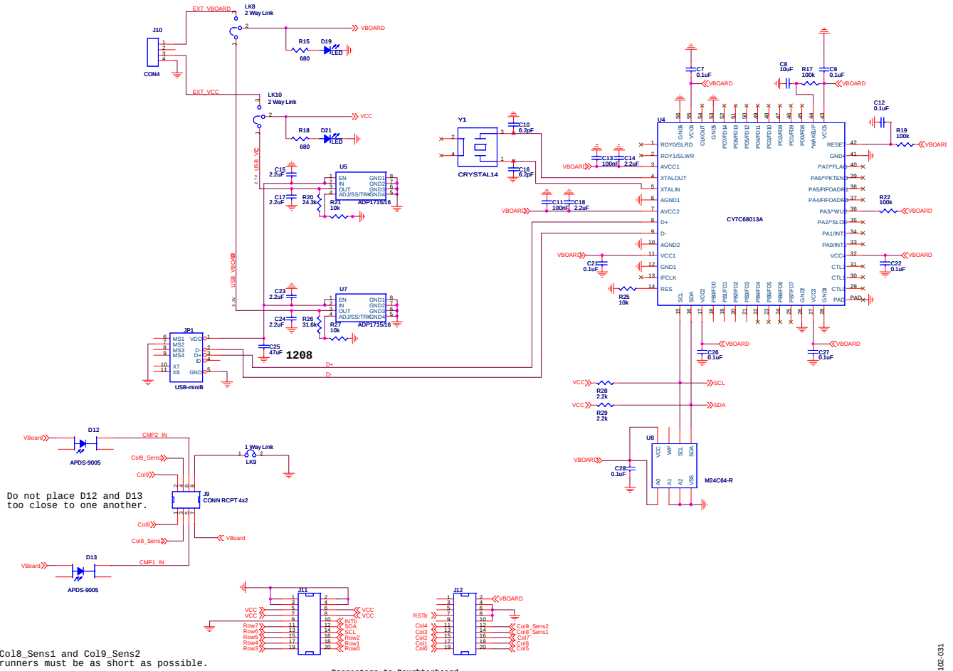
Figure 31. Motherboard Schematic (Continued)
