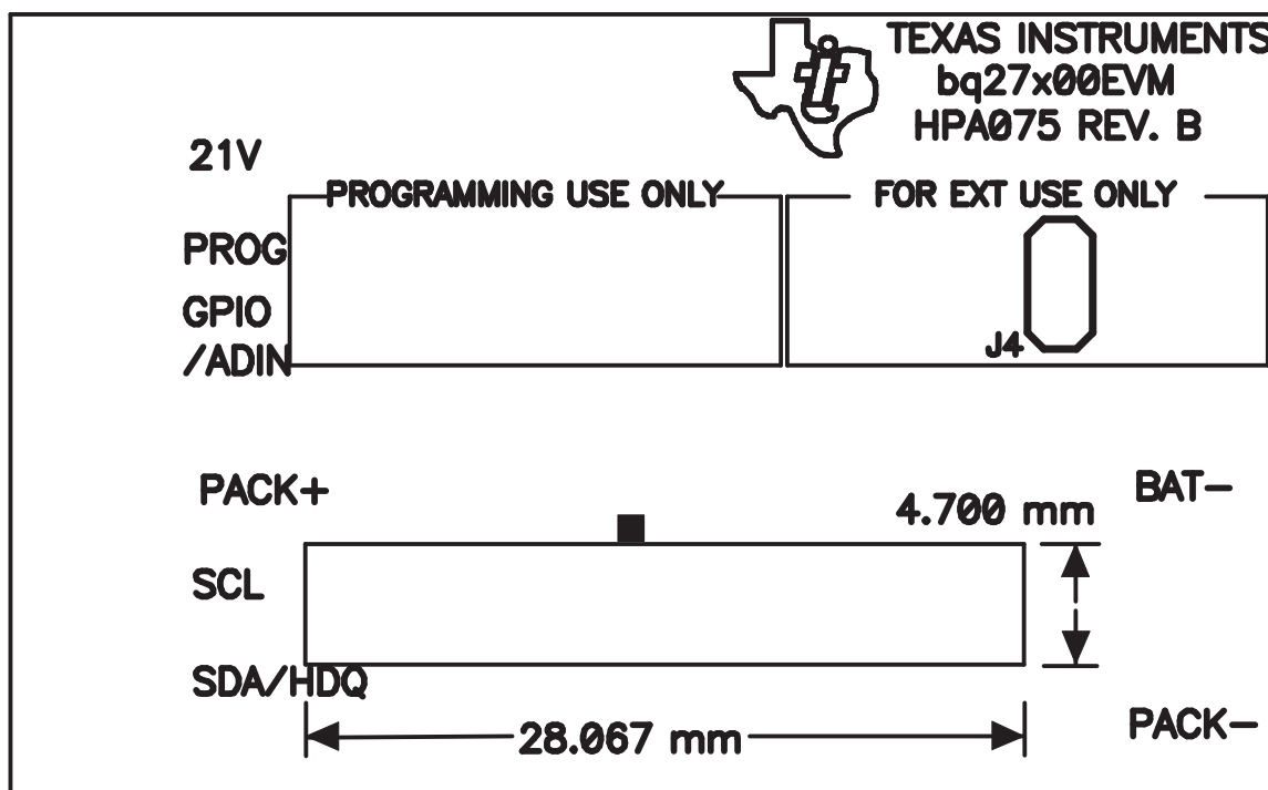
Figure 3. bq27000EVM Silkscreen
