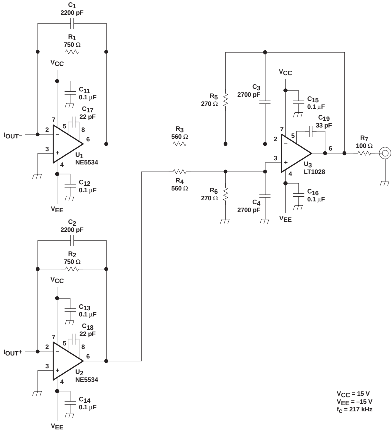
Figure 36. Measurement Circuit for PCM, V_{OUT} = 2\ \text{V rms}
