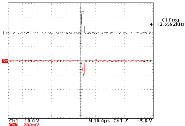
Figure 26. CS Pin at Light Load Condition
