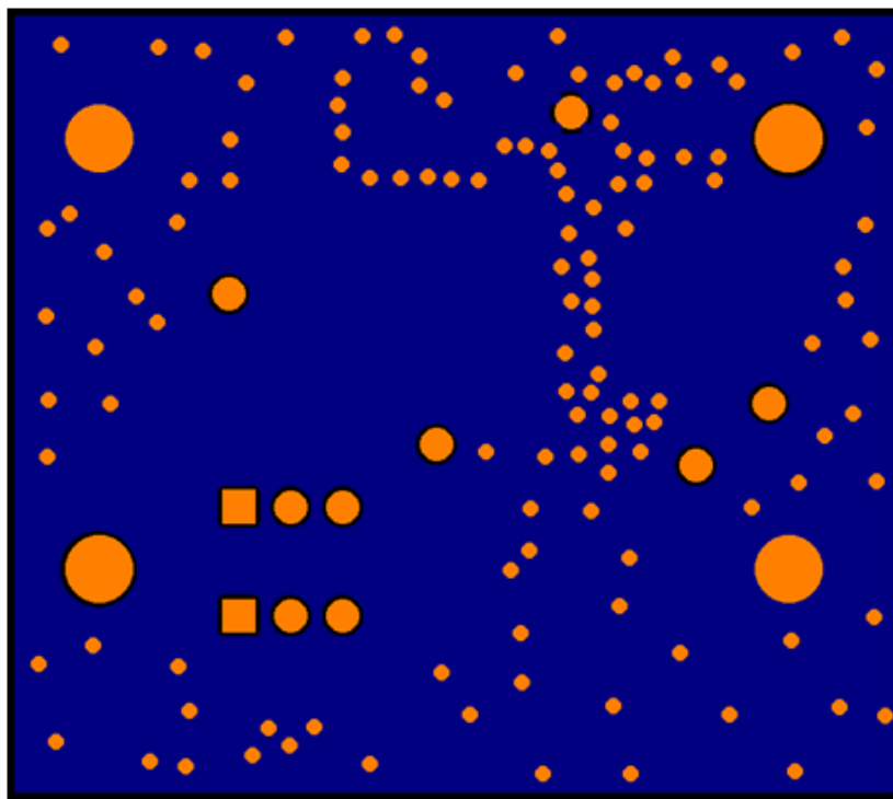
Figure 3. Bottom Layer
