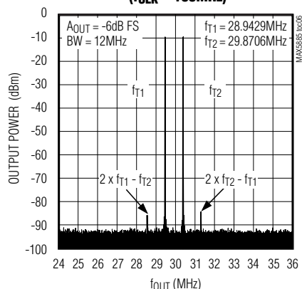
TWO-TONE INTERMODULATION DISTORTION ( f_{CLK} = 100MHz )
