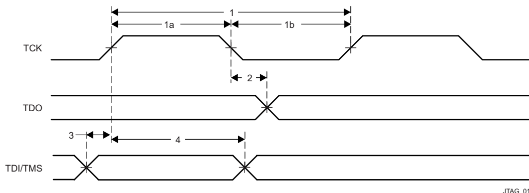
Figure 7-109. JTAG Timing
