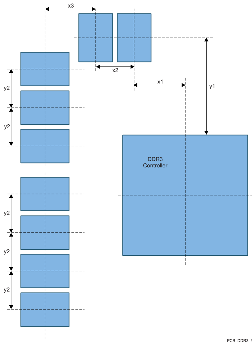
Figure 8-4. Placement Specifications
