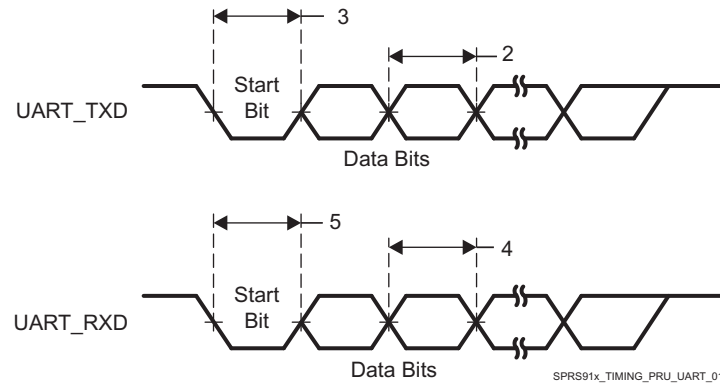
Figure 7-108. PRU-ICSS UART Timing
