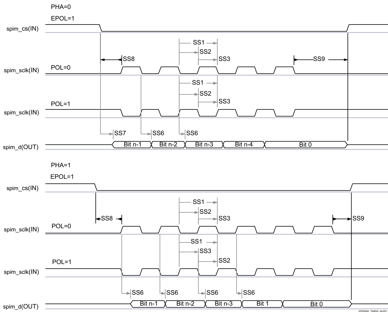
Figure 7-35. McSPI - Slave Mode Transmit
