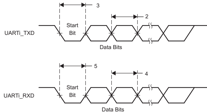
Figure 7-32. UART Timing
