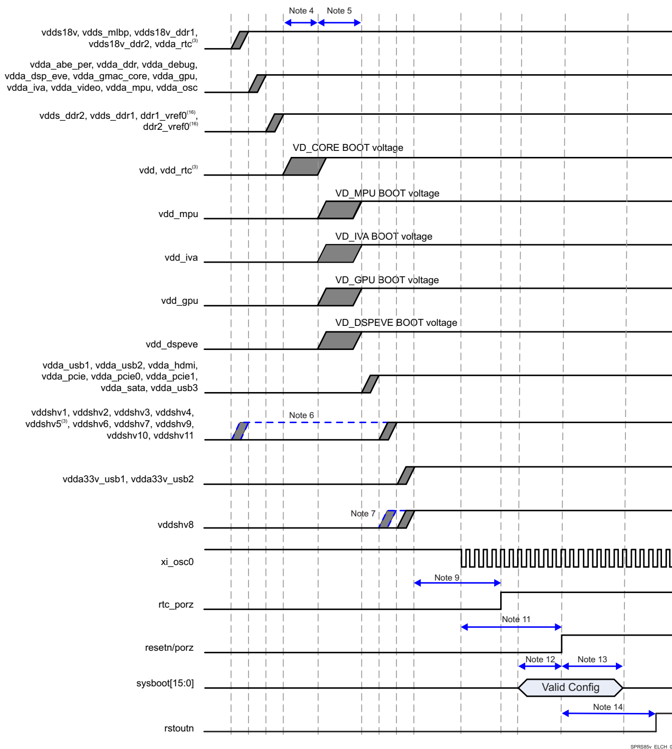
Figure 5-2. Power-Up Sequencing
