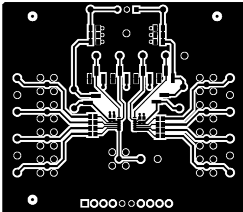
Figure 2. PCB Layer 1: Top Layer
