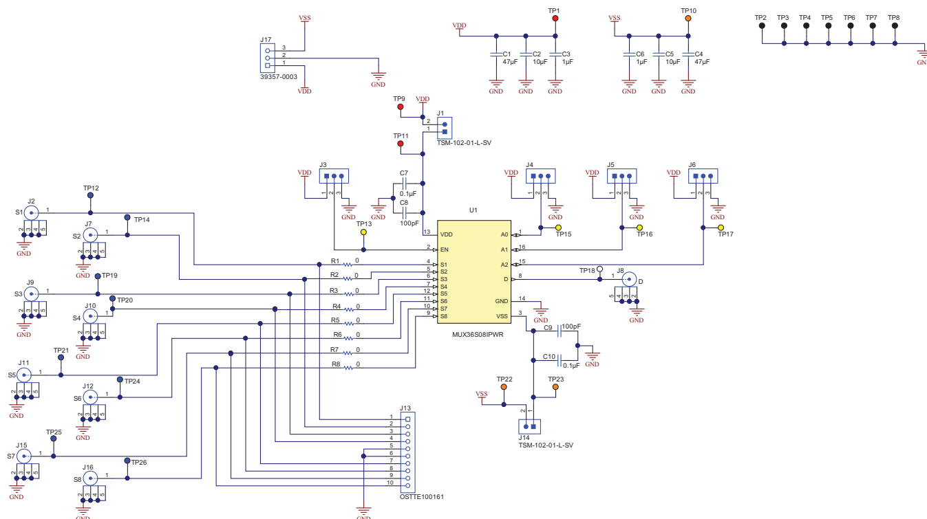
Figure 4. Schematic Diagram: Electrical
