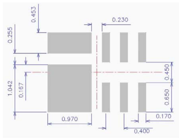
Figure 21. Footprint
