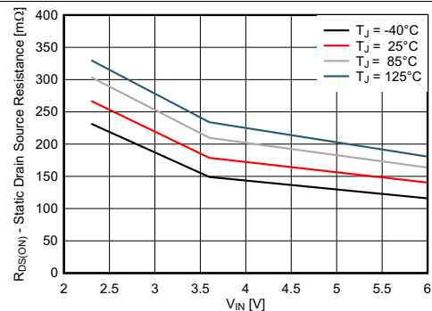
Figure 4. Low Side Switch Static Drain-Source On-State Resistance vs Input Voltage
