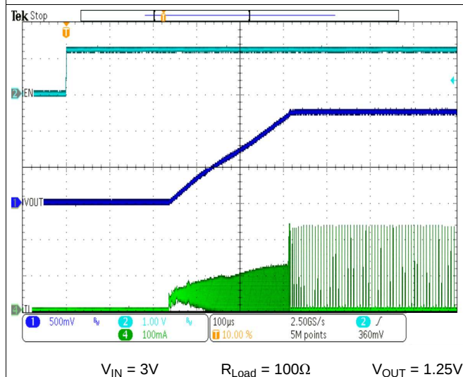
Figure 12. Start-Up Timing
