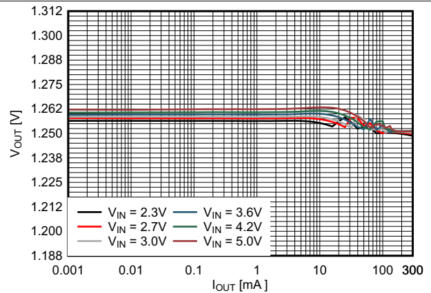
Figure 9. Output Voltage vs Output Current 1.25V V_{OUT}
