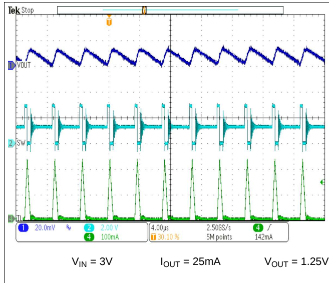
Figure 14. Typical PFM Mode Operation
