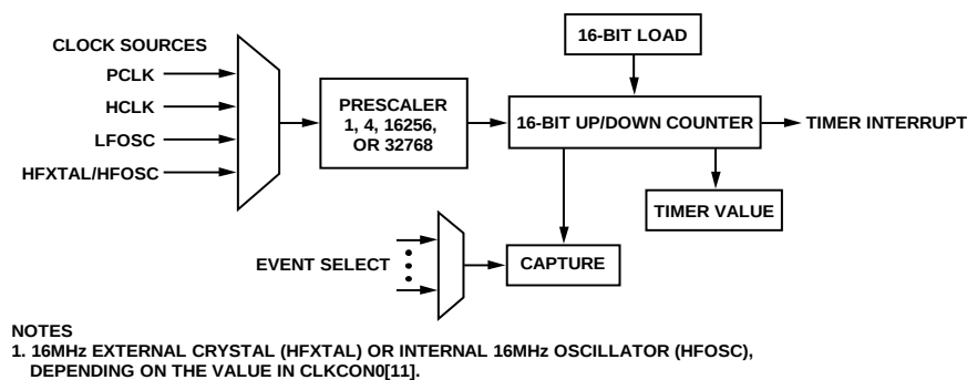
Figure 31. General-Purpose Timers Block Diagram
