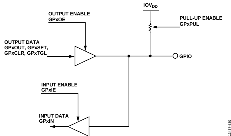
Figure 18. GPIO Structure for Port 0 to Port 3
