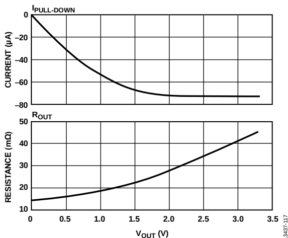
Figure 20. Typical P4 to P5 Pull-Down Characteristics
