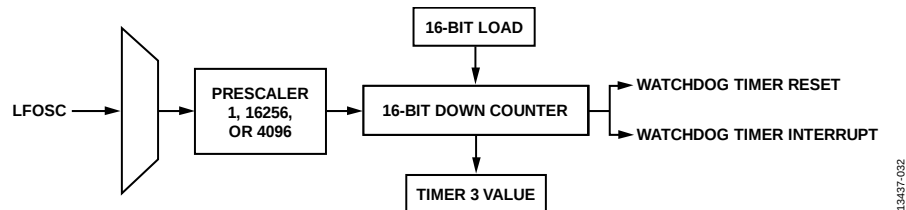
Figure 32. Watchdog Timer Block Diagram
