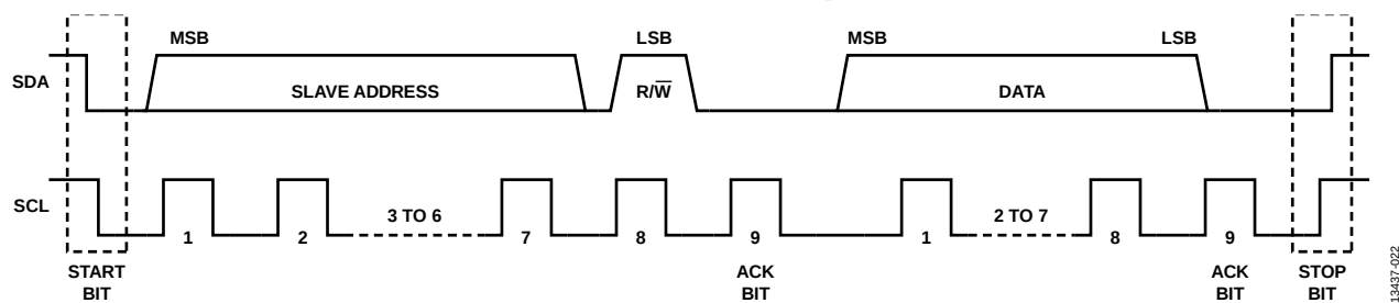
Figure 21. Typical I 2 C Transfer Sequence
