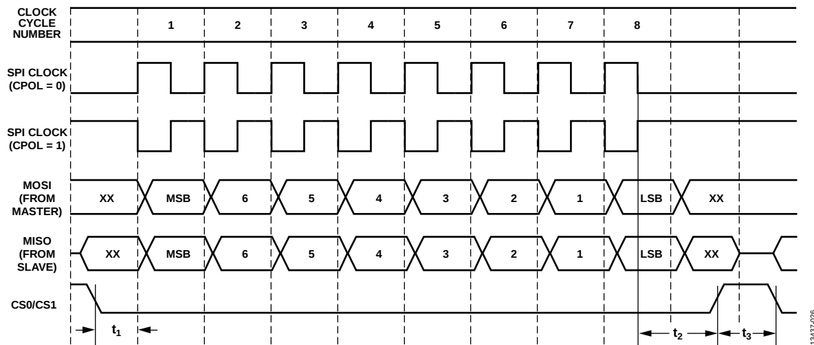
Figure 26. SPI Transfer Protocol, CPHA = 1
