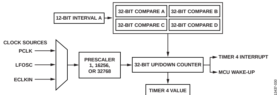
Figure 33. Wake-Up Timer Block Diagram
