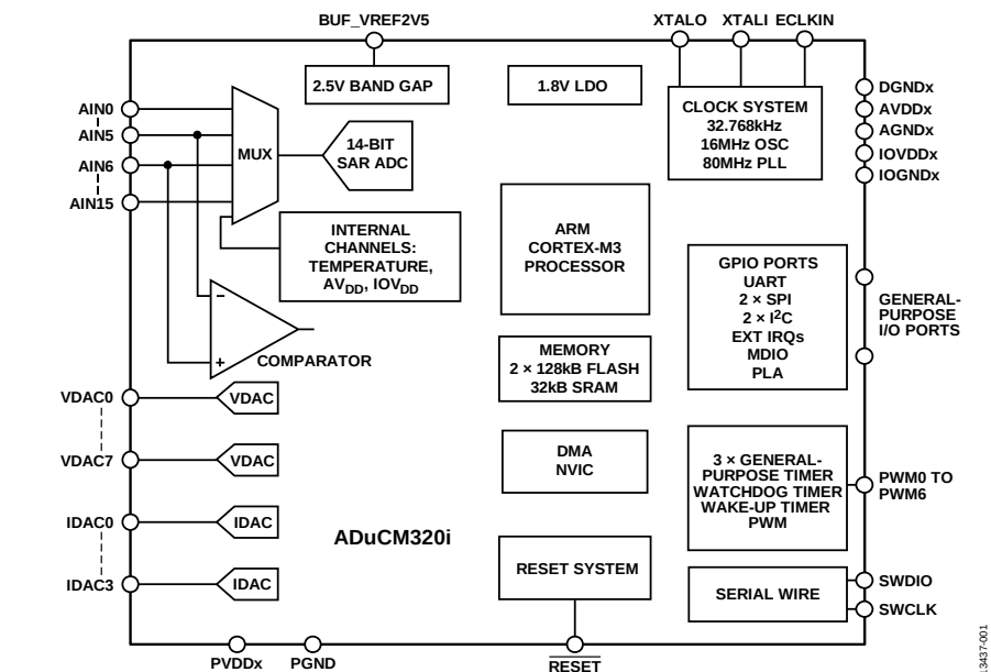
Figure 1. ADuCM320i Functional Block Diagram
