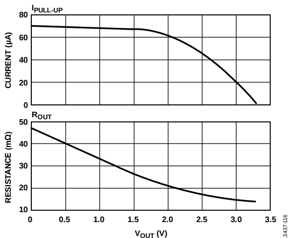
Figure 19. Typical P0 to P3 Pull-Up Characteristics
