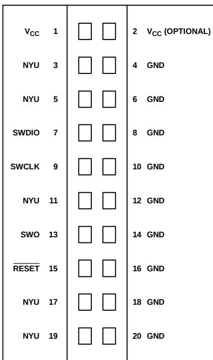
Figure 45. SWD 20-Pin Connector Pinout
