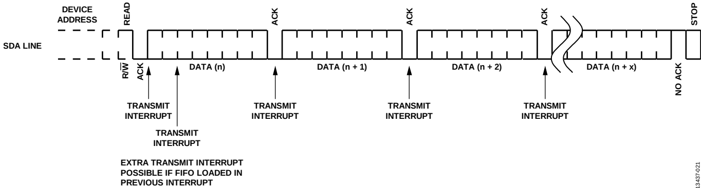
Figure 24. I²C Slave Tx Interrupt Details
