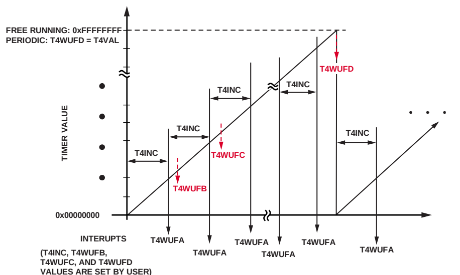
Figure 34. Wake-Up Timer Fields Action
