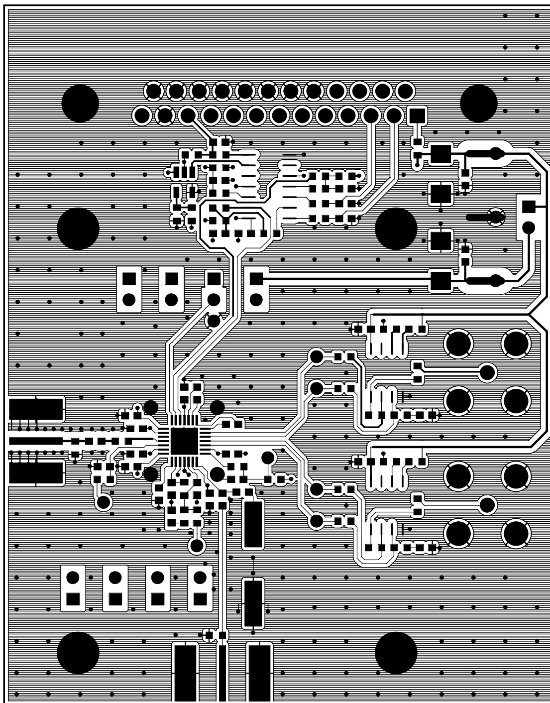
Figure 3. MAX2120 EV Kit PCB Layout—Top
