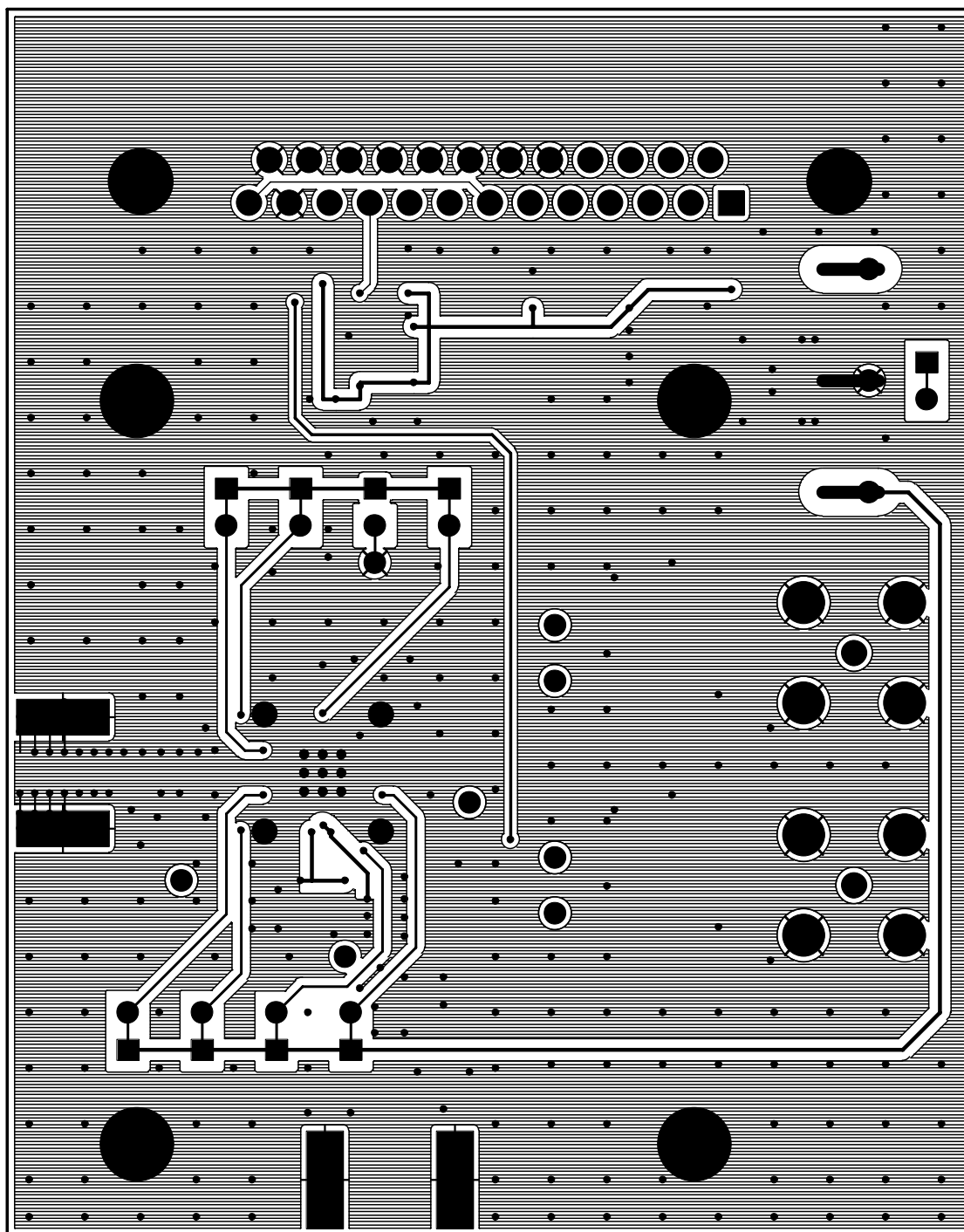
Figure 4. MAX2120 EV Kit PCB Layout—Bottom
