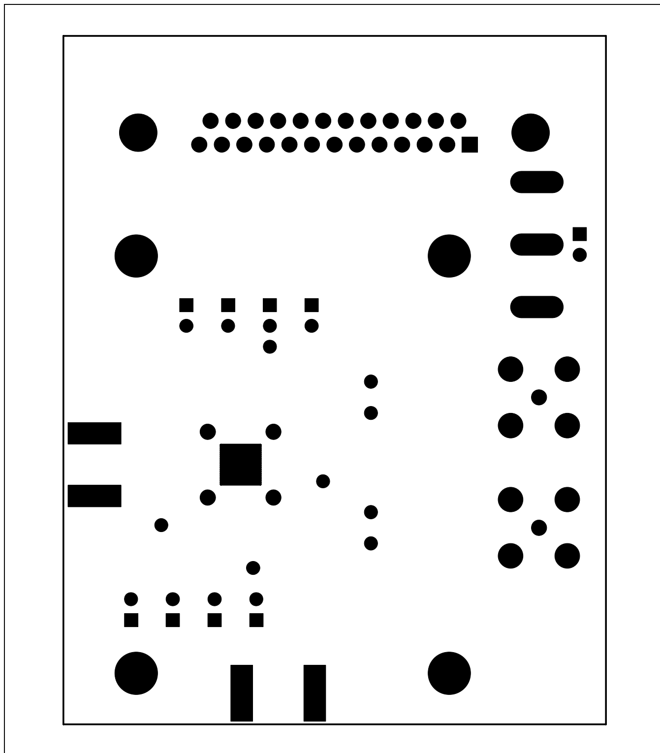
Figure 6. MAX2120 EV Kit PCB Layout—Bottom Soldermask
