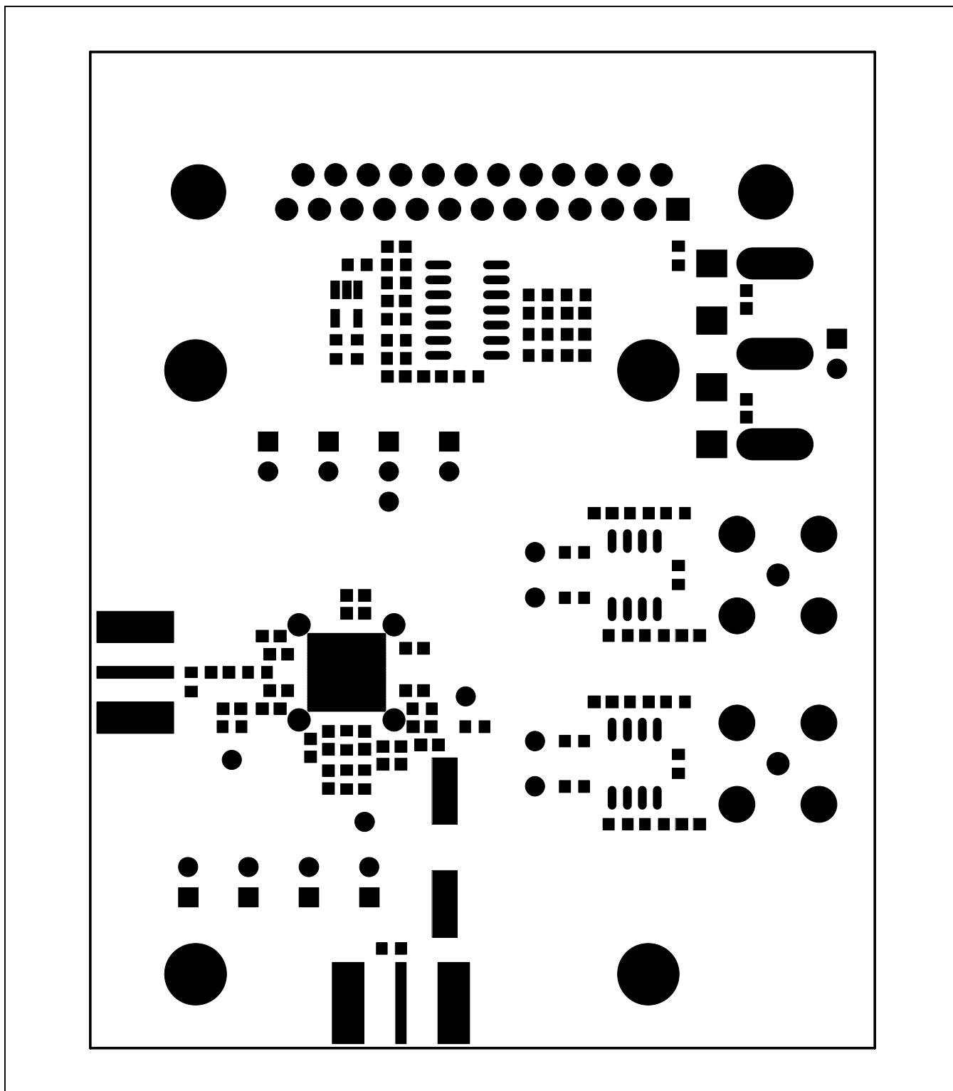
Figure 5. MAX2120 EV Kit PCB Layout—Top Soldermask
