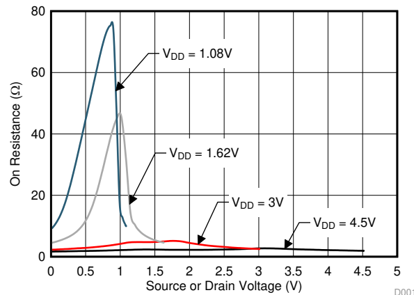
Figure 19. On-Resistance vs Source or Drain Voltage
