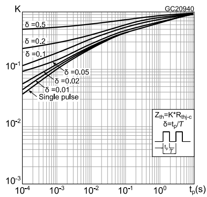
Figure 28: Thermal impedance for diode
