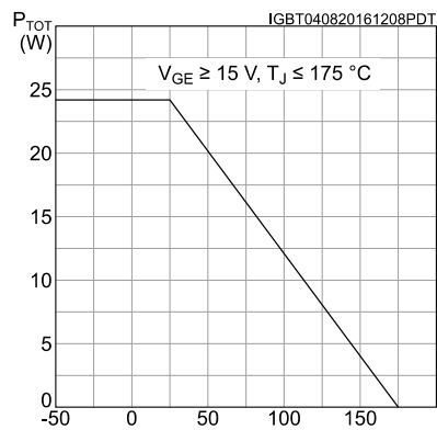
Figure 2: Power dissipation vs. case temperature
