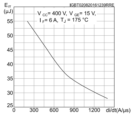
Figure 26: Reverse recovery energy vs. diode current slope
