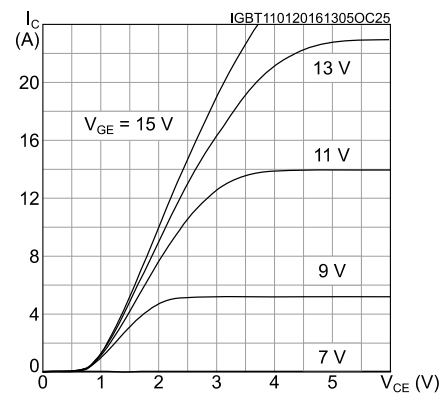
Figure 4: Output characteristics ( T_J = 25 \text{ }^{\circ}\text{C} )
