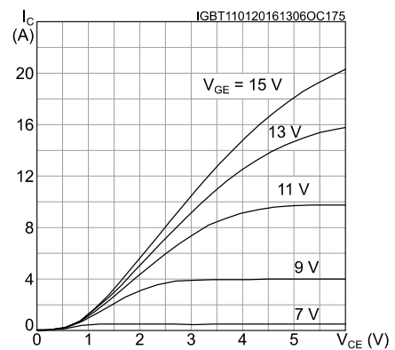
Figure 5: Output characteristics ( T_J = 175 \text{ }^{\circ}\text{C} )
