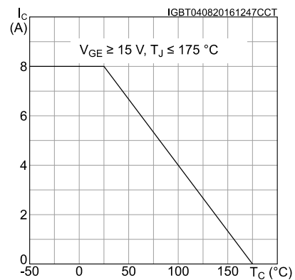
Figure 3: Collector current vs. case temperature
