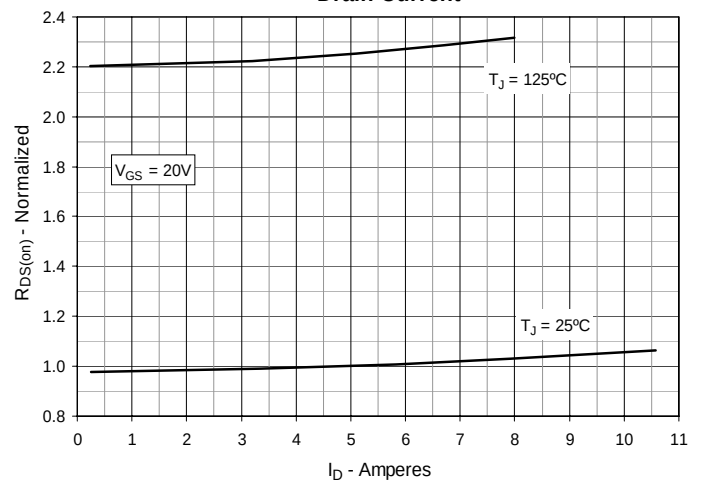
Fig. 4. R_{DS(on)} Normalized to I_D = 4\text{A} Value vs. Drain Current
