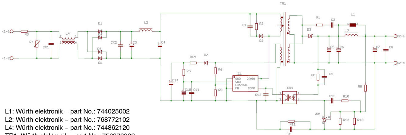
Figure 1. Circuit Diagram
