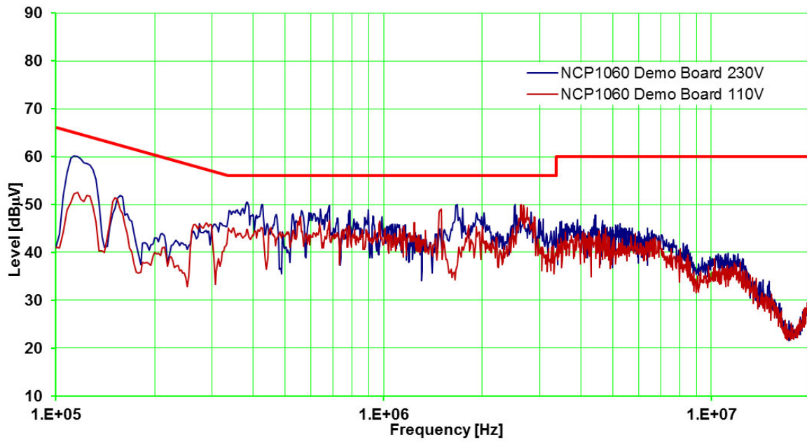
Figure 4. Conducted Emission Quasi-peak dBμV (Domestic)
