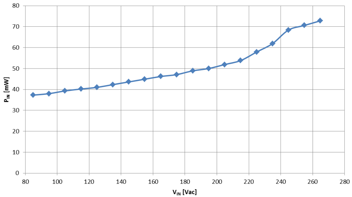
Figure 6. No-load Power Consumption vs. Line Input Curves
