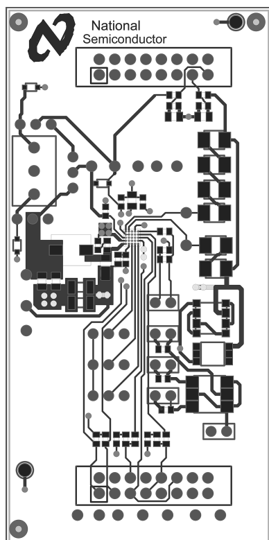
Figure 11. LP5526 Evaluation Board Layer 1 (Top, Signal)
