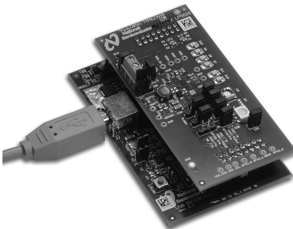
Figure 1. LP5526 Evaluation Board with USB Interface Board
