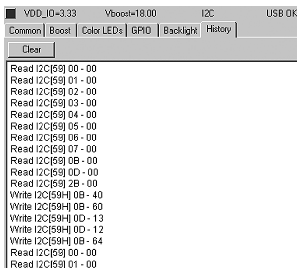
Figure 7. History Tab
