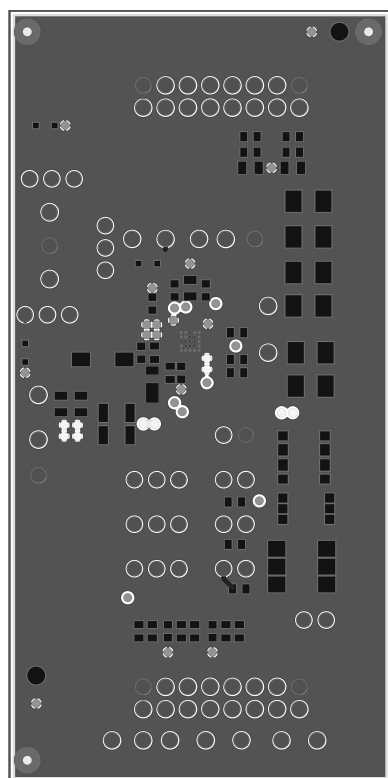
Figure 13. LP5526 Evaluation Board Layer 3 (GND)
