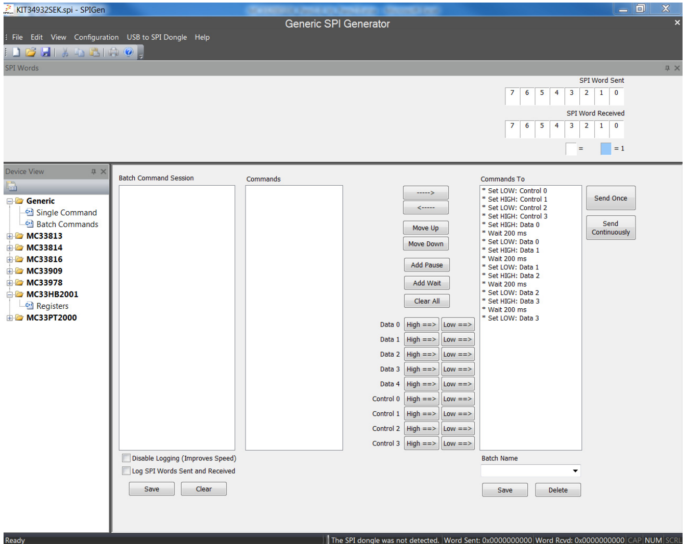
Figure 8. SPIGen GUI
