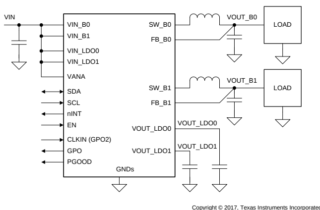
Simplified Schematic
