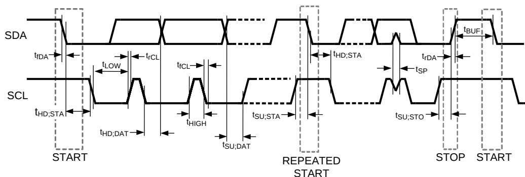
Figure 21. I²C-Compatible Timing
