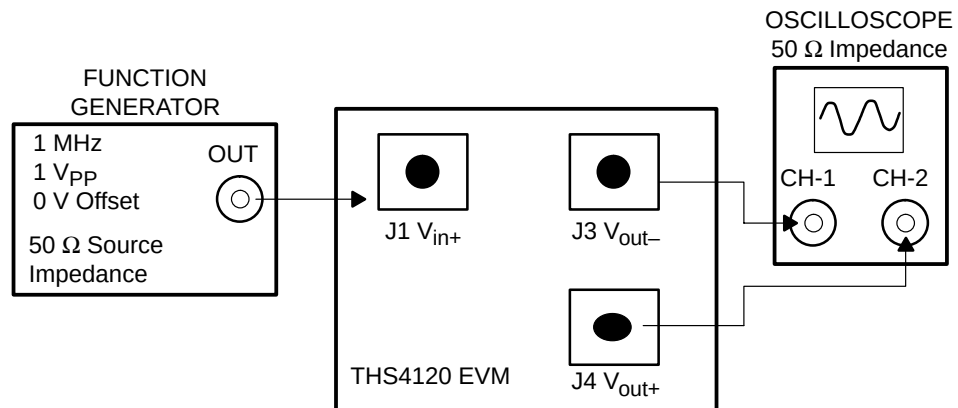
Figure 2–2. Signal Connections
