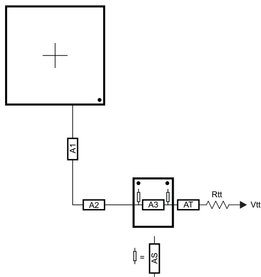
Figure 8-72. ADDR_CTRL Routing for Two Mirrored DDR3 Devices
