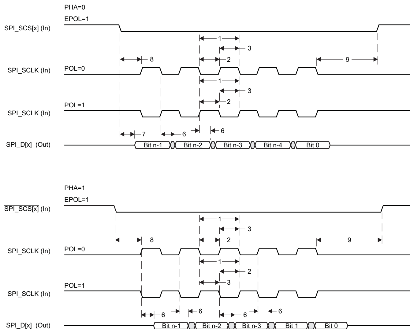
Figure 8-95. SPI Slave Mode Transmit Timing
