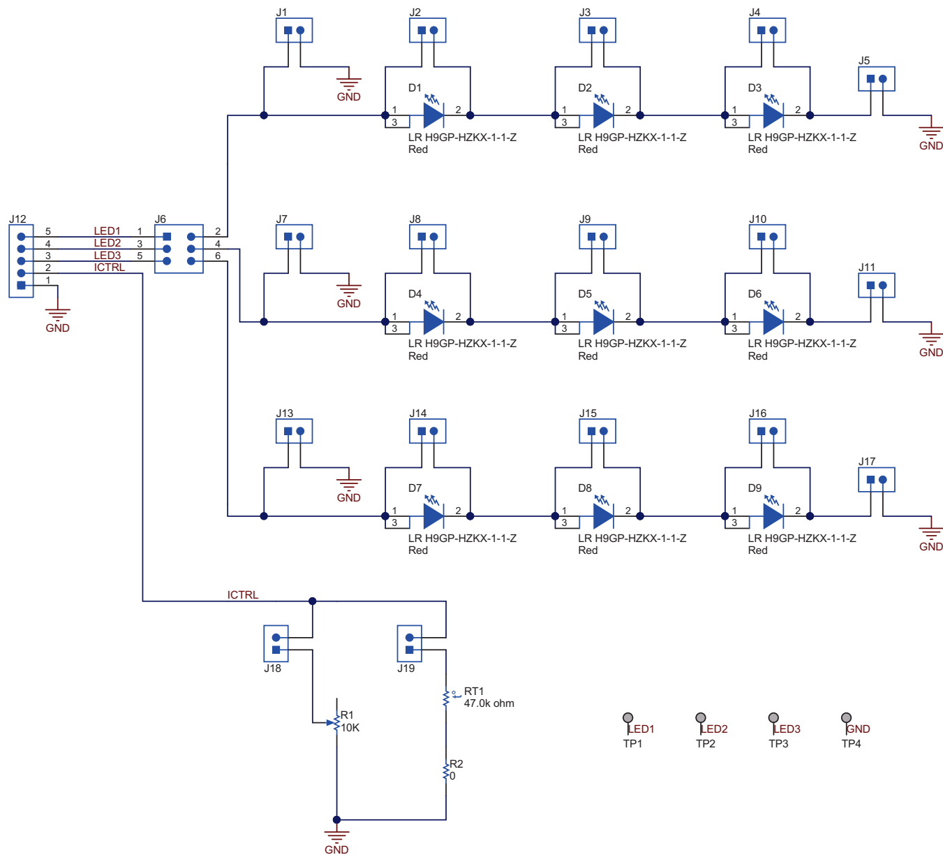
Figure 7. LED Board Schematic
