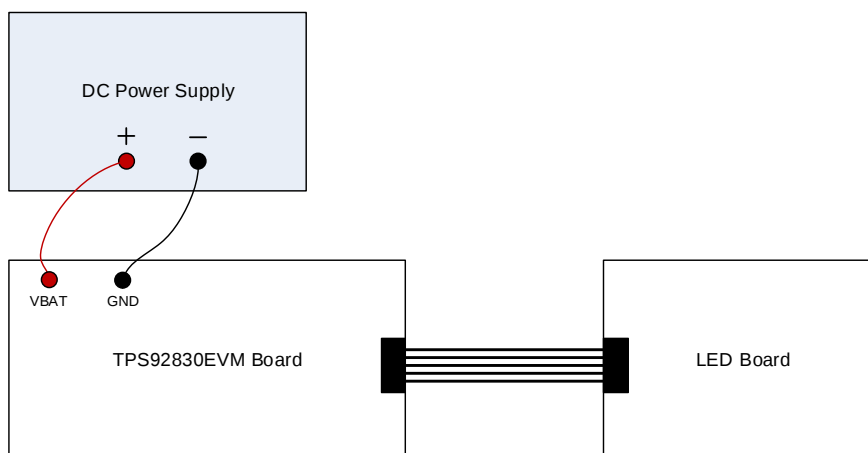
Figure 3. TPS92830EVM Setup
