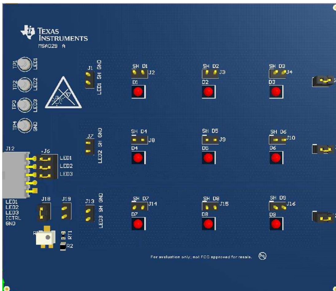
Figure 2. LED Board
