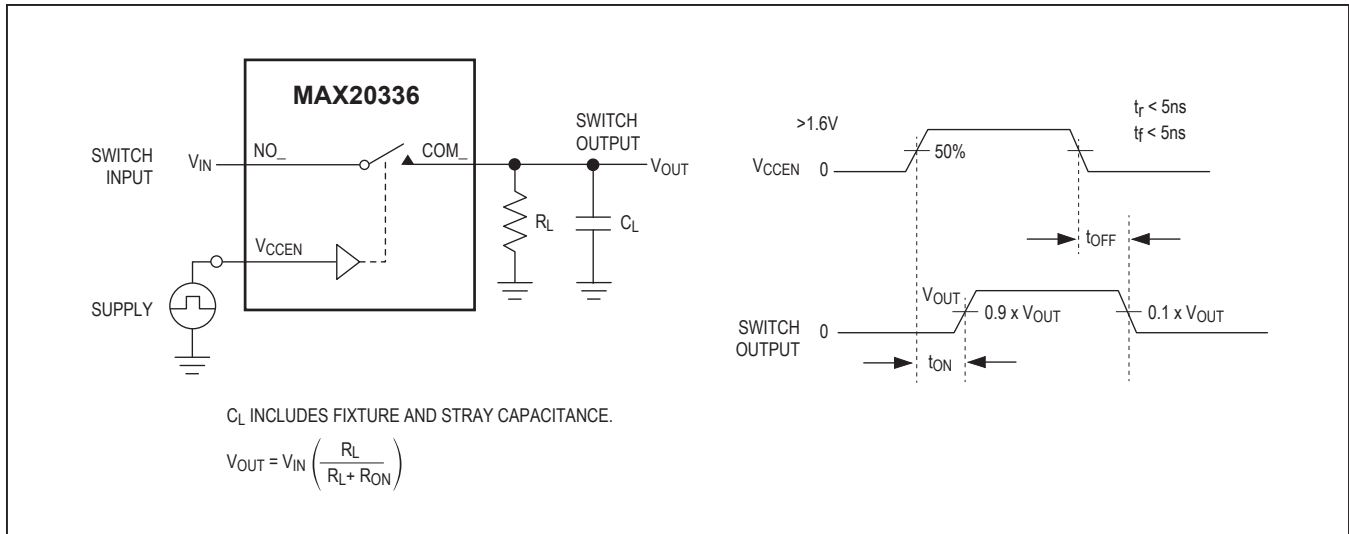
Figure 1. Switching Time
