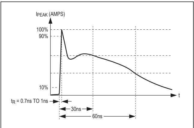
Figure 6. IEC 61000-4-2 ESD Generator Current Waveform
