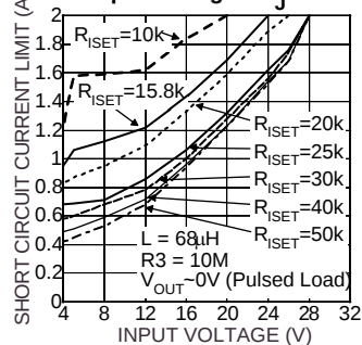
Short Circuit Current Limit vs. Input Voltage at T_J = 85^\circ\text{C}
