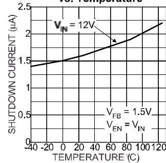
Shutdown Current vs. Temperature
