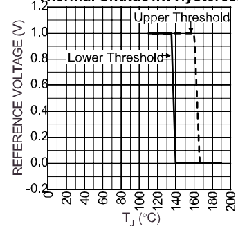
Thermal Shutdown Hysteresis
