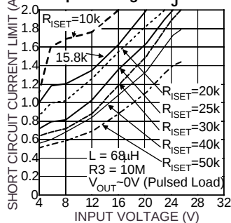
Short Circuit Current Limit vs. Input Voltage at T_J = 125^\circ\text{C}
