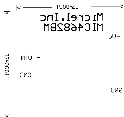
Figure 5d. Bottom Silkscreen
