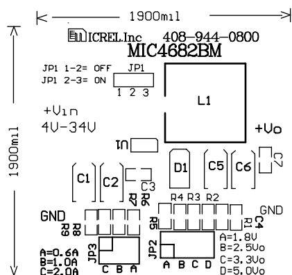
Figure 5b. Top Silkscreen
