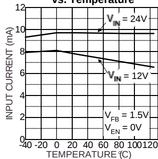
Quiescent Current vs. Temperature
