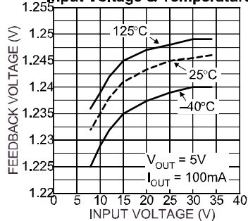
Feedback Voltage vs. Input Voltage & Temperature
