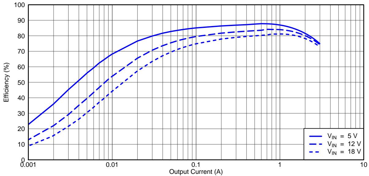
Figure 4. TPS542941EVM Converter 2 Light Load Efficiency
