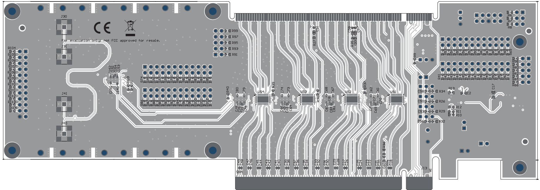
Figure 6. Bottom Layer
