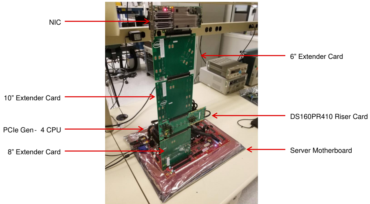
Figure 3. Example Test Setup
