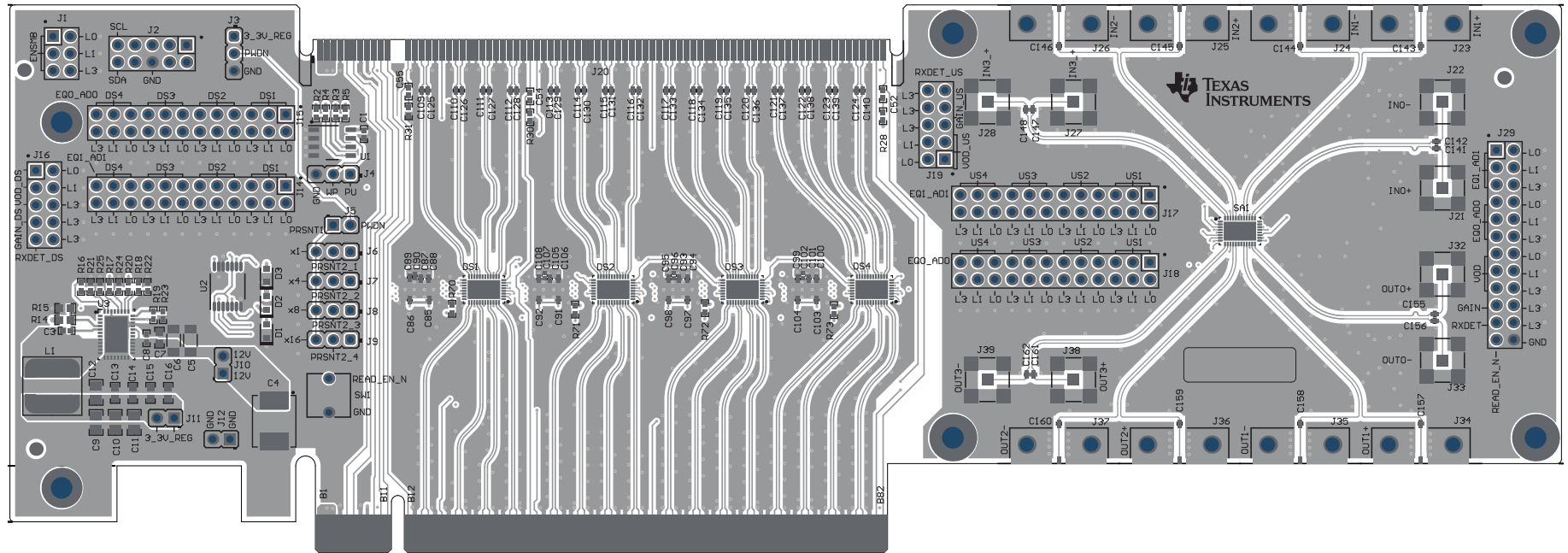
Figure 5. Top Layer
