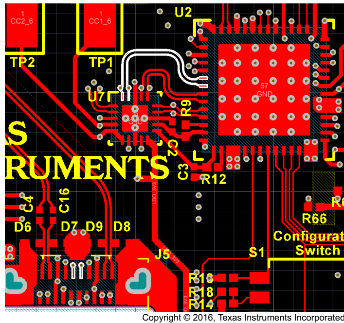
Figure 90. Top Layer Component Routing
