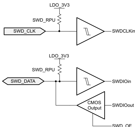
Figure 60. IOBUF_GPIOHSSWD
