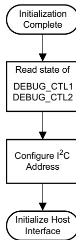
Figure 62. I²C Address Configuration
