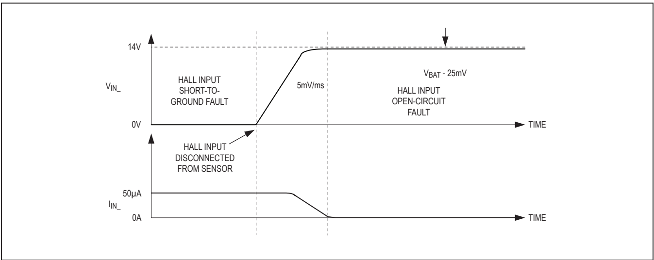
Figure 3. Hall Input Ramps to Open-Circuit Fault When a Short to Ground Is Relieved
