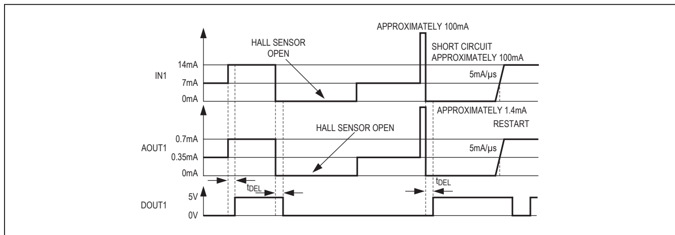
Figure 1. Timing Diagram
