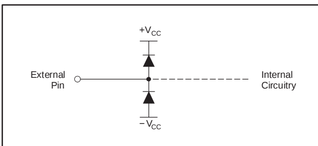
Figure 11. Internal ESD Protection
