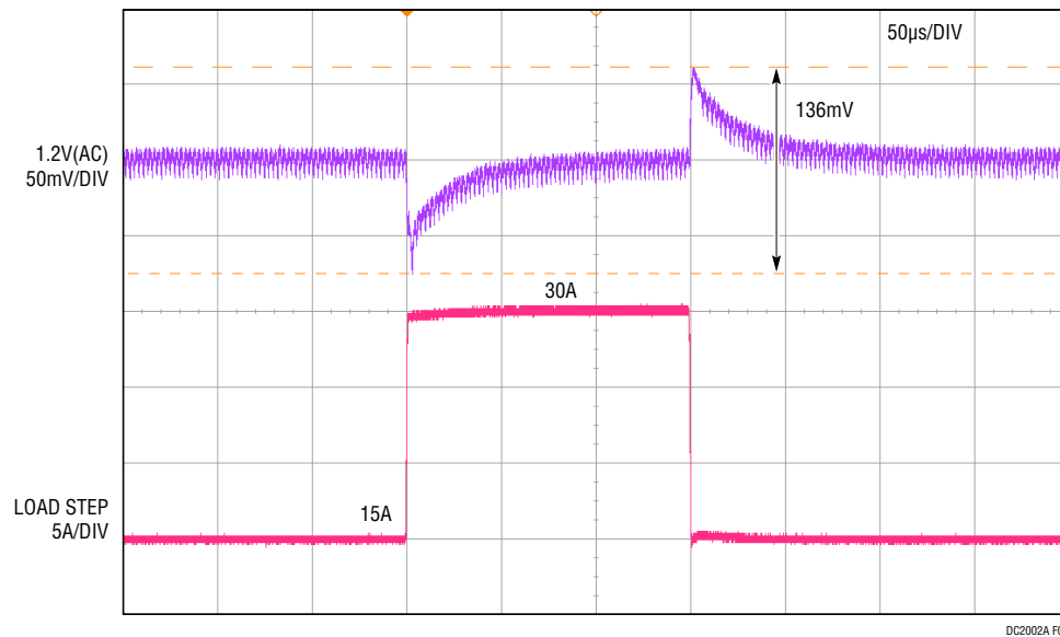
Figure 5. 50% to 100% to 50% Load Step Response of the 1.2V Rail. C_{OUT} = 3 \times \text{Sanyo 2R5TPE330M9} \parallel 2 \times 100\mu\text{F X5R 1206} , L = \text{Würth 744301033 (0.33}\mu\text{H)} , f_{SW} = 400\text{kHz} .
