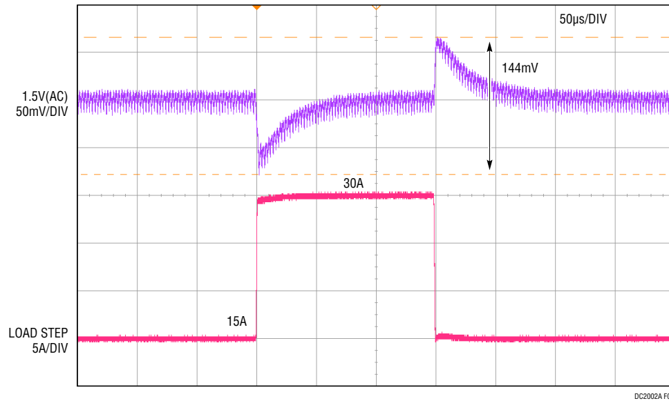
Figure 4. 50% to 100% to 50% Load Step Response of the 1.5V Rail. C_{OUT} = 3 \times \text{Sanyo 2R5TPE330M9} \parallel 2 \times 100\mu\text{F X5R 1206} , L = \text{Würth 744301033 (0.33}\mu\text{H)} , f_{SW} = 400\text{kHz} .
