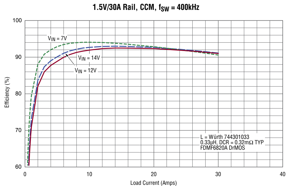
Figure 2. Efficiency Curves for the 1.5V Rail at V_{IN} = 12V, 14V and 7V in CCM.
