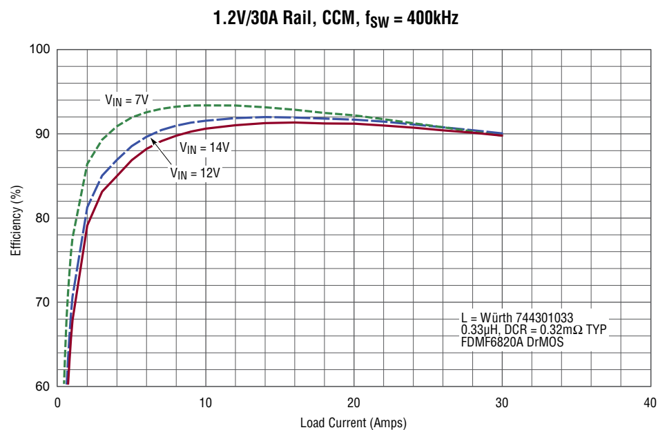
Figure 3. Efficiency Curves for the 1.2V Rail at V_{IN} = 12V, 14V and 7V in CCM.
