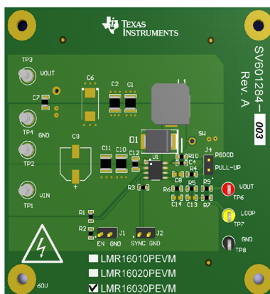
Figure 1. LMR16030PEVM Board
