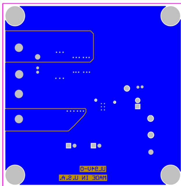
Figure 6. Bottom Layer
