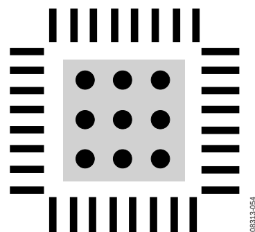
Figure 56. Exposed Pad Layout Example, Top View
