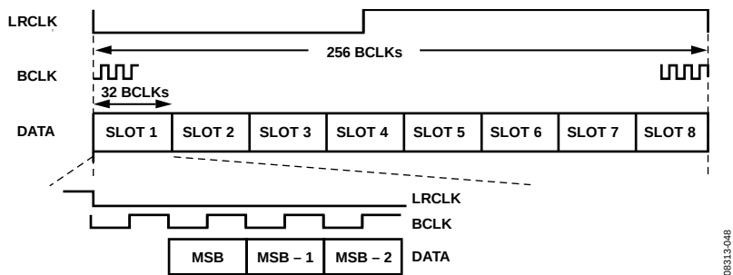
Figure 50. TDM Mode
