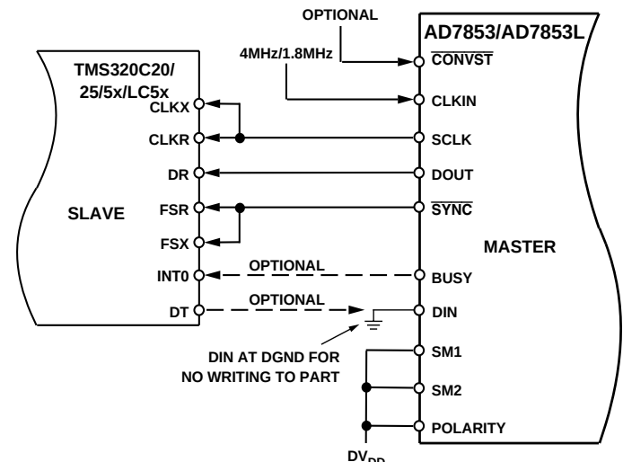
Figure 49. TMS320C20/25/5x Interface
